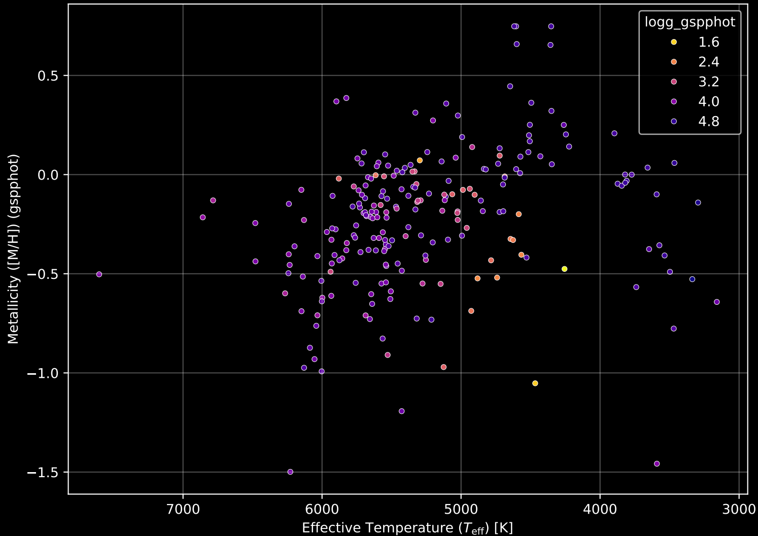
APOGEE DR17 Field: [045-54-O] Stellar Population Parameters (n= 226)
