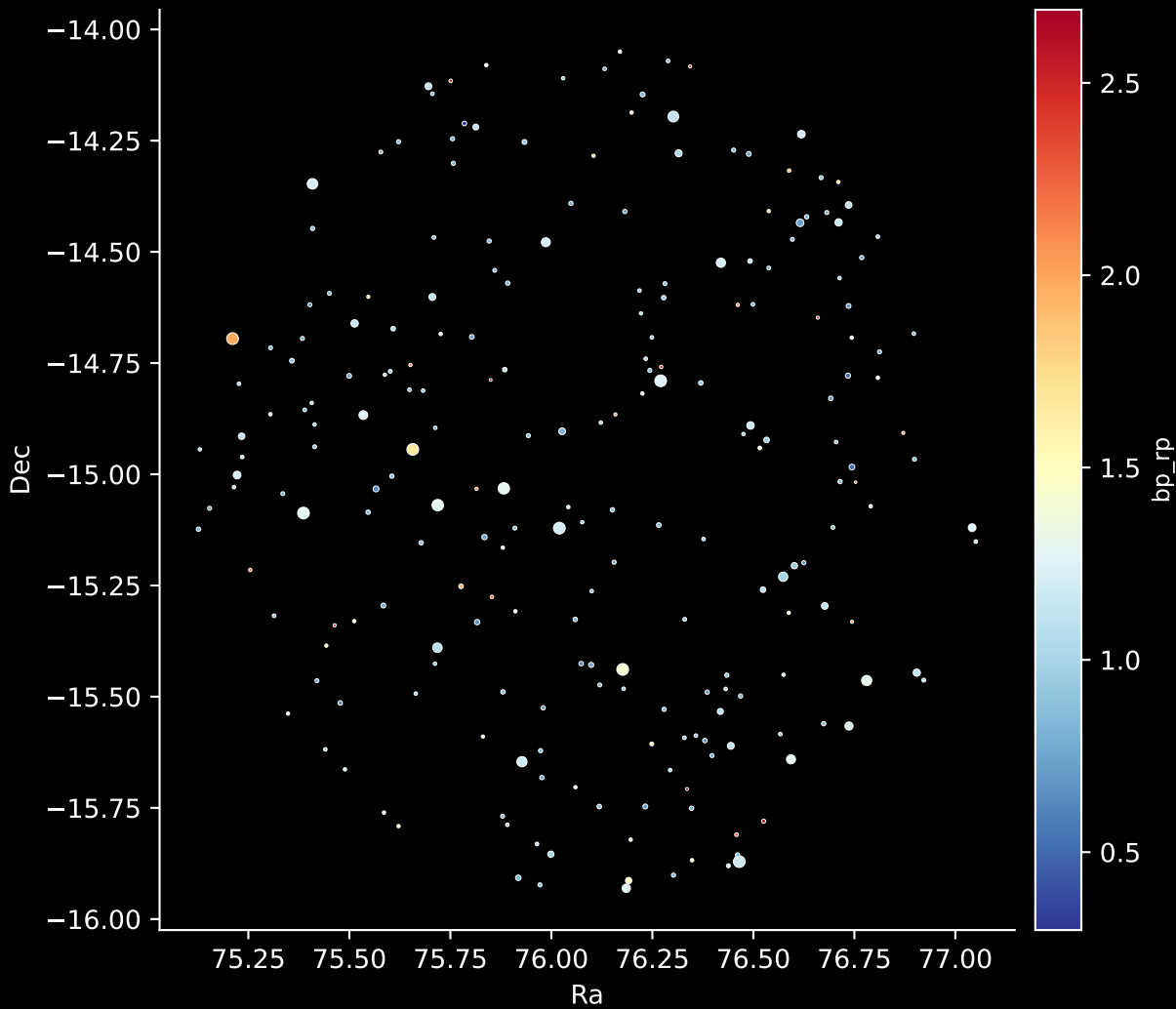
APOGEE DR17 Field: [045-54-O] Stars: 226
