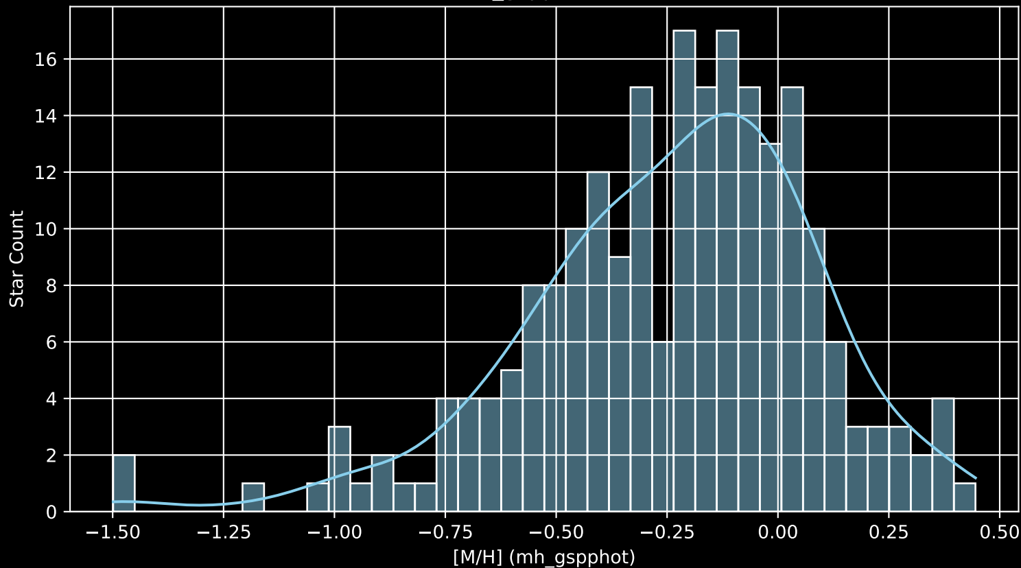
APOGEE DR17 Field: [045-54-O [M/H] (mh_gspphot) (n= 221)
