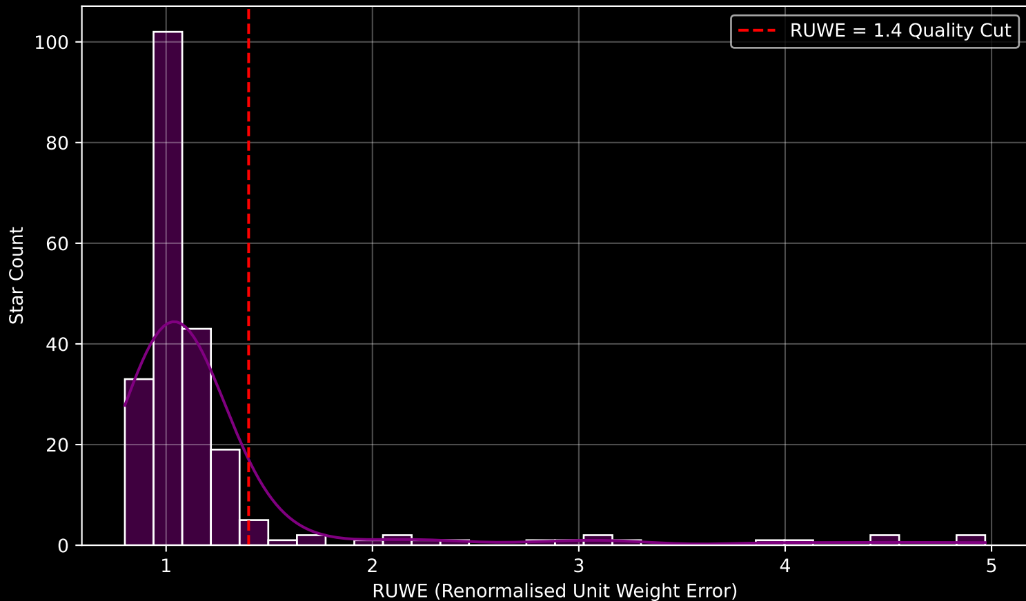
GAPOGEE DR17 Field [045-54-O] RUWE Distribution (n= 221)
