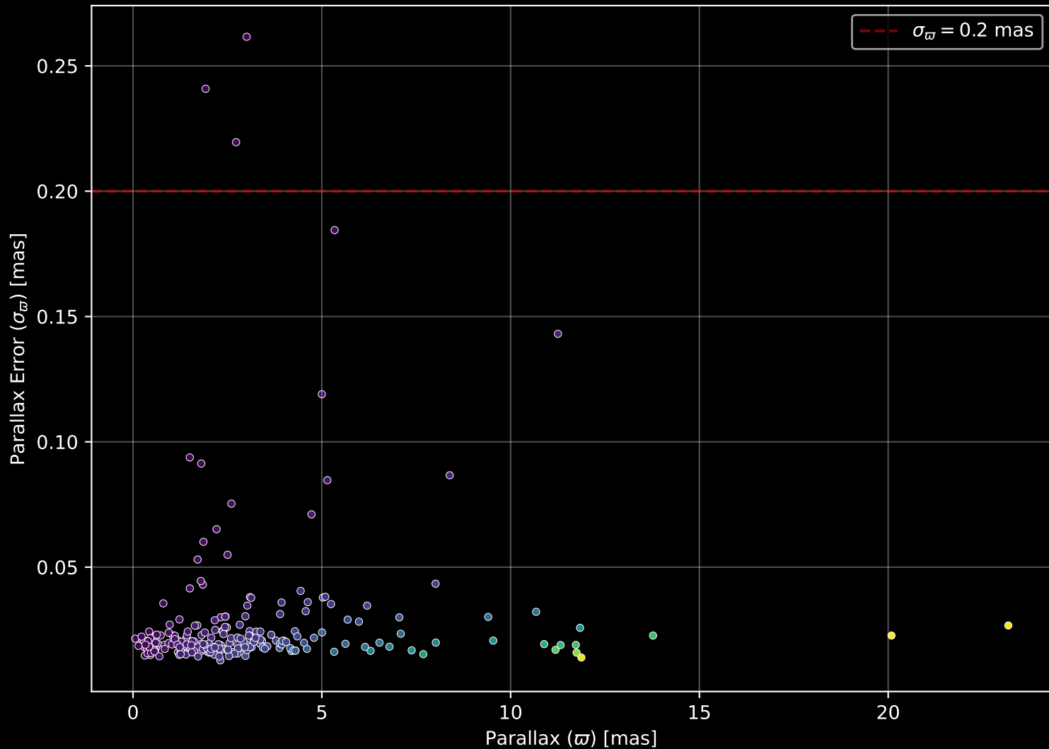
APOGEE DR17 Field: [045-54-O] Parallax Quality (n= 226)
