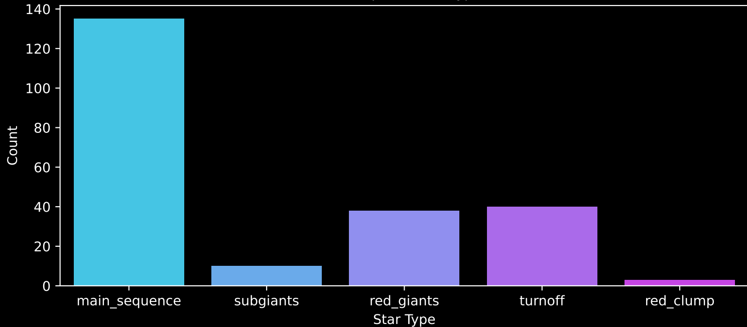
APOGEE DR17 Field: [045-54-O] Count plot of Star Type
