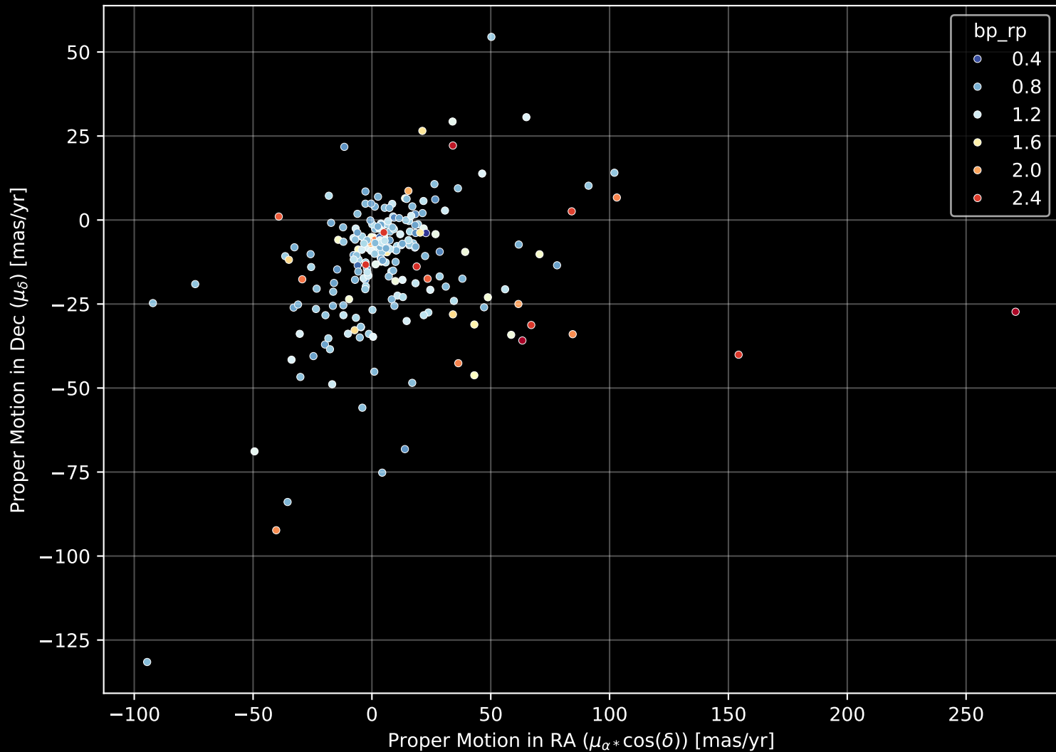
APOGEE DR17 Field: [045-54-O] Proper Motion Diagram (n= 226)
